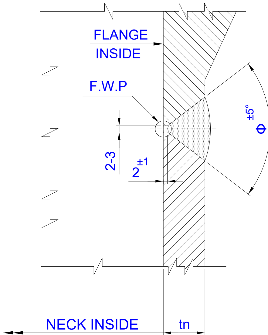
WELD DETAIL OF FLANGE TO NOZZLE NECK
